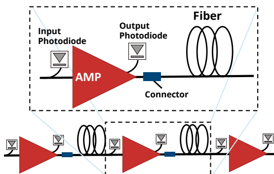
Figure 1. Line system scheme
