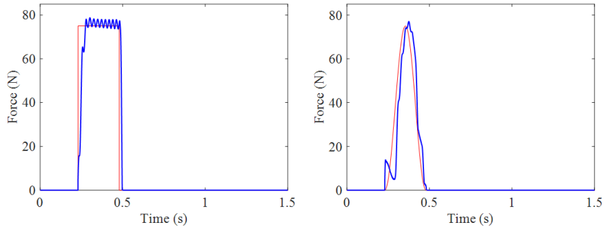
Figure 5.8: Force tracking performance for simulations carried out with two reference profiles lasting 250 ms with 75 N amplitude.
