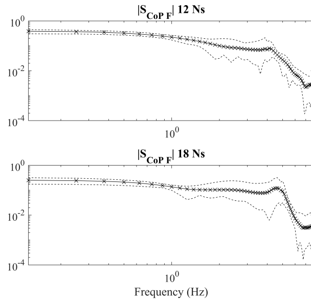
Figure 7.22: Magnitude of input sensitivity functions of CoP displacement with respect to perturbation force for an adult subject, 58 years old, BMI 19.0. Average FRFs for 12 N s and 18 N s stimuli are shown in solid lines, minimum and maximum FRFs are presented with dashed lines.
