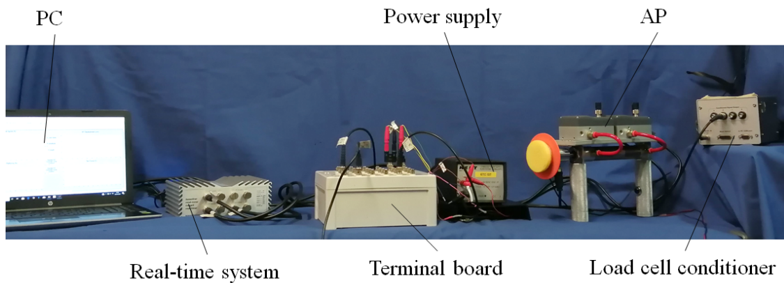
Figure 6.3: Main components of the final perturbation system.
