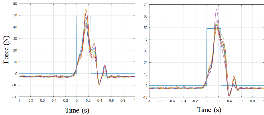
Figure 3.10: Force tracking in hand-held condition during experimental trials on healthy subjects. Thoracic stimuli on the left, lumbar stimuli on the right.
