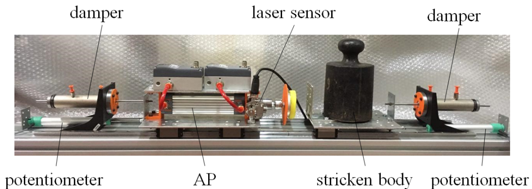
Figure 5.2: The experimental test-bench.
