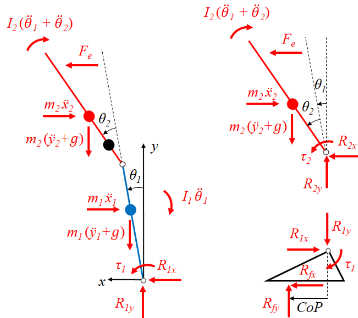
Figure 7.3: Free body diagrams of double link inverted pendulum model for postural analysis. Dot notation represents time derivative.
