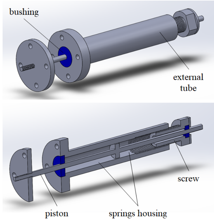
Figure 5.4: Custom-built visco-elastic damper.
