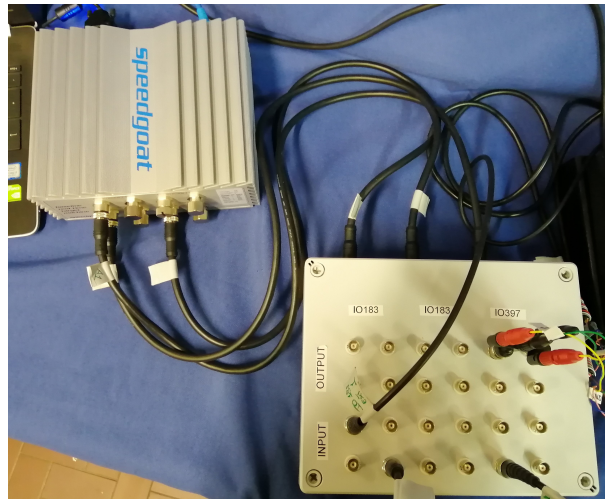
Figure 5.3: Real-time system (Speedgoat GmbH, Germany) and terminal box.
