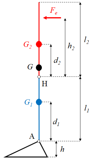
Figure 7.2: Representation of double link inverted pendulum model for postural analysis; blue and red segments represent respectively lower limb and trunk.
