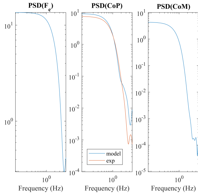
Figure 7.37: Power spectral density of force perturbation (left), CoP displacement (center) and CoM displacement (right), double link inverted pendulum model, subject 4.
