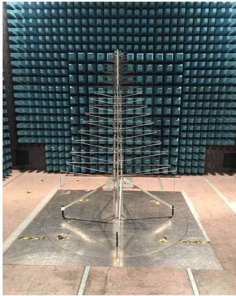
FIGURE 10. Antenna under test in a semi-anechoic chamber. The dimensions of the chamber (9.10 x 5.80 x 5.55 m) are not adequate for measuring the antenna pattern. The main purpose of the chamber is to embed the antenna in a RF quiet environment, where the absorbing walls act as a blackbody emitting at room temperature.
