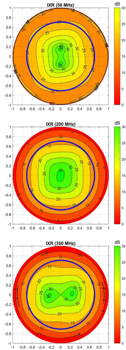
FIGURE 9. uv -maps maps of the IXR for y -polarization at 50, 200 and 350 MHz. The color map has been saturated to highlight low IXR values. The blue circle indicates the edge of the FoV.
