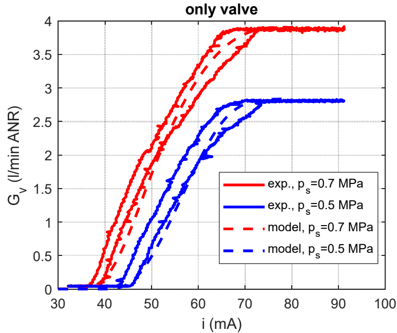
Figure 17: Air flow through the valve vs input current; comparison between experimental and numerical results
