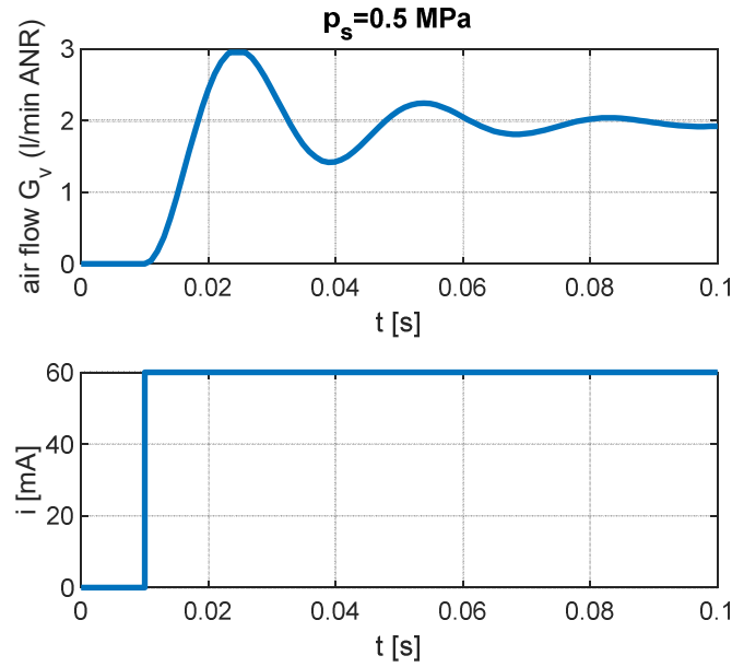
Figure 16: Valve response to a step in input current with p_s=0.5 MPa
