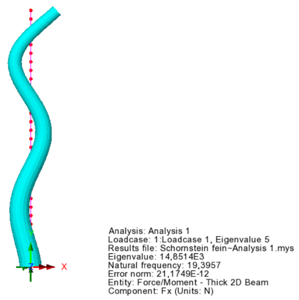
Fig. 9.4: Fourth natural frequency
