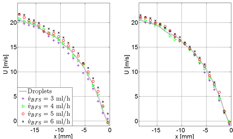
Fig. 4 Time averaged streamlines at U_{\infty} = 30 m/s obtained with micron-size droplets and HFSB with four different volume rates of BFS and two volume rates of helium: \dot{v}_{He} = 4 l/h (left), \dot{v}_{He} = 5 l/h (right). Streamlines determined by cross-correlation analysis
