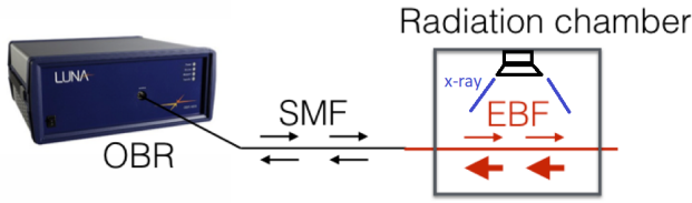
Fig. 2. Schematic representation of the measurement setup. OBR=Optical Backscattering Reflectometer. SMF=Single Mode Fiber. EBF=Enhanced Back-scattering Fiber. The arrows represent the optical signals propagating through the fibers.
