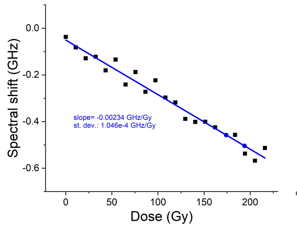
Fig. 8. Spectral shift versus accumulated dose at 22 Gy/min.
