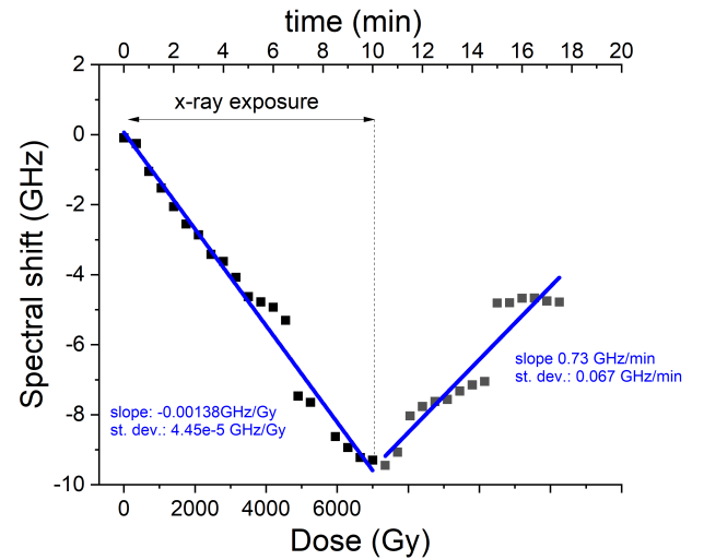
Fig. 4. Spectral shift versus exposure time and corresponding dose.
