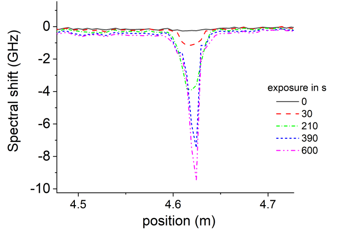
Fig. 3. Spectral shift versus position along the fiber for different times of exposure at 700 Gy/min. The spatial resolution of the data is 5 mm.
