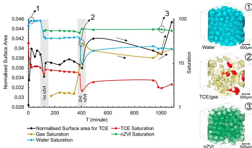
Fig. 3. Fluid phase saturation and the normalized surface area for the TCE phase within the imaged section of the bead pack as a function of time. The 3D renderings displayed at Right show fluid distributions within the FoV. TCE, red; gas, yellow; water, blue; and nZVI, green.
