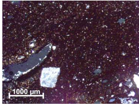
Fig. 18. Bricks of the frame of the openings (image at the optical microscope in thin section, polarised light), (Rescic).
