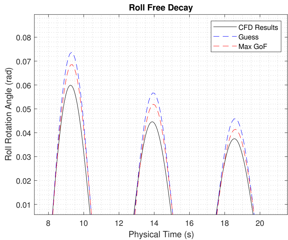
Figure 28. Large oscillations in roll.
