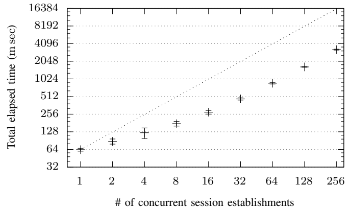
Fig. 5. Evaluation of the time required to concurrently complete multiple session establishments varying the handshake parallelism (the dotted line represents a reference corresponding to a linear increase in the elapsed time).
