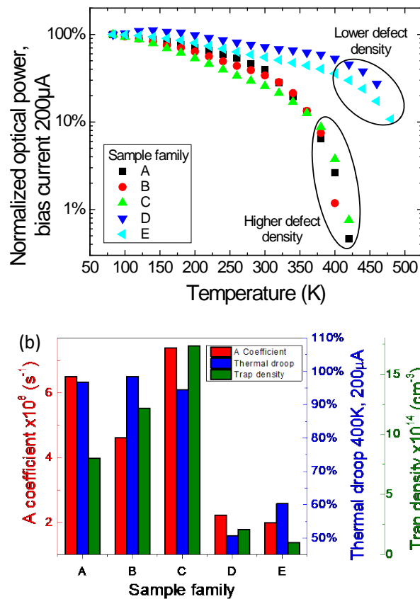
Figure 21: (a) optical power variation detected in SQW LEDs in a wide temperature range, for a representative 200 \mu A bias current. (b) the amount of thermal droop is directly correlated to the density of deep levels detected by C-DLTS and differential carrier lifetime measurements. Reprinted from C. De Santi, M. Meneghini, M. La Grassa, B. Galler, R. Zeisel, M. Goano, S. Dominici, M. Mandurrino, F. Bertazzi, D. Robidas, G. Meneghesso, and E. Zanoni, “Role of
