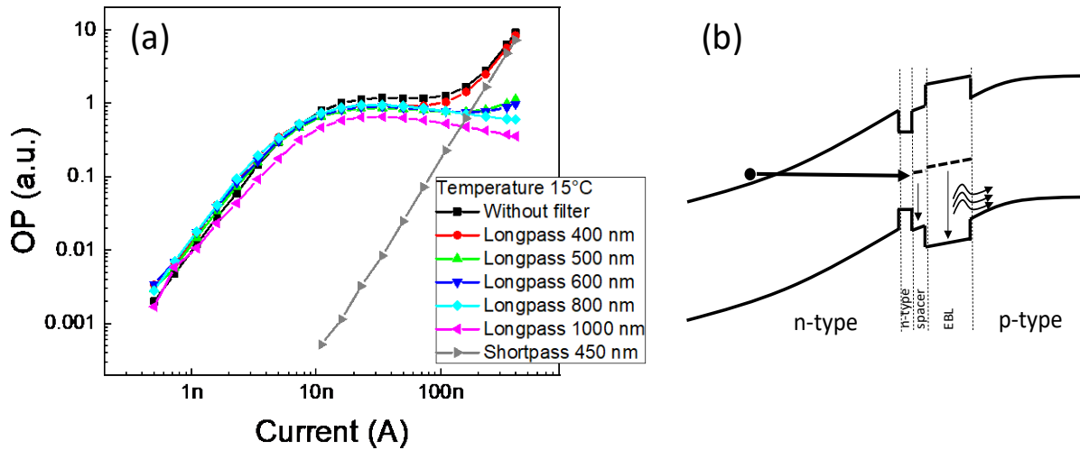
Figure 26: (a) tests carried out by varying long-pass filter cutoff frequency, to identify the dominant deep level energy. (b) summarizes the possible emission processes. Reprinted from C. De Santi, M. Buffolo, N. Renso, A. Neviani, G. Meneghesso, E. Zanoni, and M. Meneghini, “Evidence for defect-assisted tunneling and recombination at extremely low current in InGaN/GaN-based LEDs,” Appl. Phys. Express , vol. 12, no. 5, p. 052007, May 2019, DOI: 10.7567/1882-0786/ab10e3. Copyright (2019) The Japan Society of Applied Physics.
