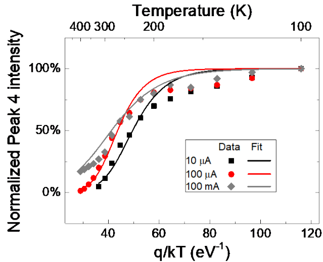
Figure 31: summary of the temperature and bias dependence of peak 4 emission, including fit according to the SRH model. Reprinted from C. De Santi, M. Meneghini, D. Monti, J. Glaab, M. Guttmann, J. Rass, S. Einfeldt, F. Mehnke, J. Enslin, T. Wernicke, M. Kneissl, G. Meneghesso, and E. Zanoni, “Recombination mechanisms and thermal droop in AlGaN-based UV-B LEDs,” Photonics Res. , vol. 5, no. 2, pp. A44--A51, Apr. 2017, DOI: 10.1364/PRJ.5.000A44. © 2017 CLP.
