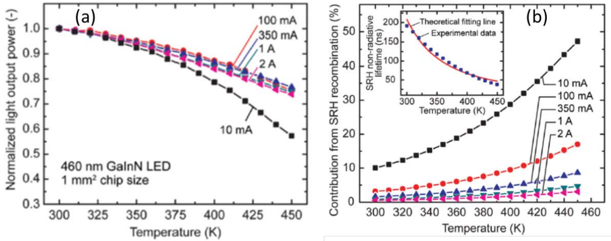
Figure 7: (a) Normalized light output power as a function of temperature at several operating points. (b) Fraction of SRH non-radiative recombination at different current levels. SRH non-radiative lifetime as a function of temperature and theoretical fit is shown in the inset. Reprinted from D. S. Meyaard, Q. Shan, J. Cho, E. Fred Schubert, S.-H. Han, M.-H. Kim, C. Sone, S. Jae Oh, and J. Kyu Kim, “Temperature dependent efficiency droop in GaInN light-emitting diodes with different current densities,” Appl. Phys. Lett. , vol. 100, no. 8, p. 081106, Feb. 2012, DOI: 10.1063/1.3688041, with the permission of AIP Publishing.
