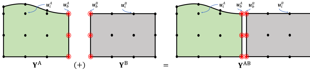
Fig. 1: A rigid coupling of two substructures A and B. The coupling exists only at the interface DoF by virtue of the compatibility condition i.e. \mathbf{u}_b^A - \mathbf{u}_b^B = \mathbf{0} . Note that the DoF of both the substructures are shown in \mathbf{Y}^{AB} signifying dual nature of the formulation.
