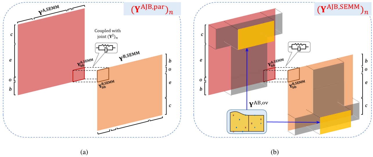
Fig. 5: A graphical representation of how the hybrid model for a coupled structure is obtained. (a) The parent model is made by coupling two hybrid models at the boundary DoF b . The DoF order for substructure B is reversed for this visual illustration. Adding a joint produces the coupled parent model (\mathbf{Y}^{\text{AJB,par}})_n at n^{\text{th}} iteration. (b) The coupled parent model together with the measurements of the assembled structure (overlay model) yields the coupled hybrid model (\mathbf{Y}^{\text{AJB,SEMM}})_n . The overlay model DoF in the full-system measurements are also shown.
