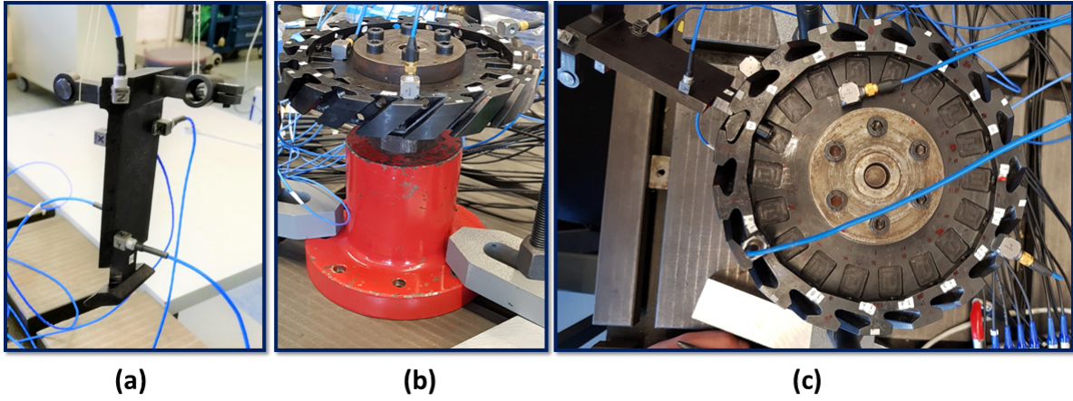
Fig. 6: The experimental setup with all the accelerometers mounted on: (a) the blade hanged by wires (b) the disk fixed at its centre (c) the coupled blade and disk with the same constraint conditions as the disk.
