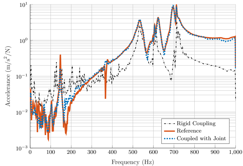
Fig. 10: The agreement of the FRF before and after identification. The solid validation line is a measured FRF of the full-system labelled "Reference" (measured on circle marked DoF in Fig. 7c). The blue dotted line indicates the coupled results (with the joint identified by the SEMM procedure). The dash-dotted black line is the would-be rigid coupling (without joint). The coupled results are in agreement with the full-system reference FRF.
