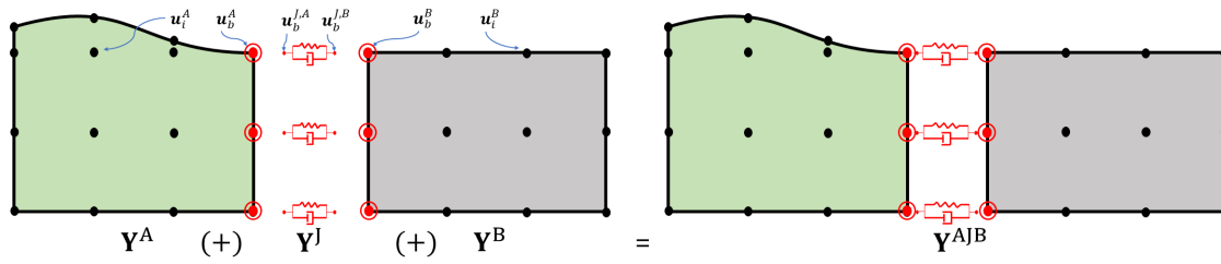
Fig. 2: Flexible coupling between substructures A and B by introducing a joint model consisting of a spring and a damper between the interface DoF of the substructures. The compatibility conditions read as \mathbf{u}_b^A - \mathbf{u}_b^{J,A} = \mathbf{0} and \mathbf{u}_b^B - \mathbf{u}_b^{J,B} = \mathbf{0} .
