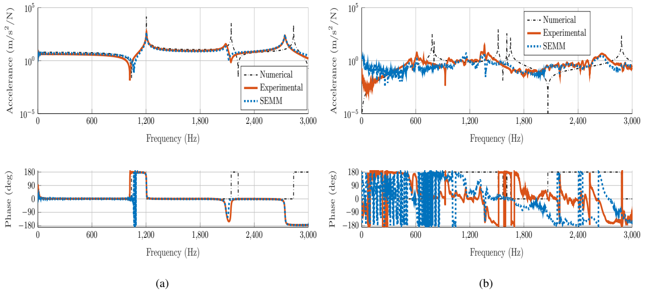
Fig. 8: FRFs for the SEMM validation of (a) Blade and (b) Disk at the DoF marked with squares in Fig. 7a and 7b, respectively. The numerical FRFs were computed without any damping. The expanded FRF (legend: SEMM) for the blade agrees well with the experimental reference; whereas for the disk, it has lesser agreement in some regions.
