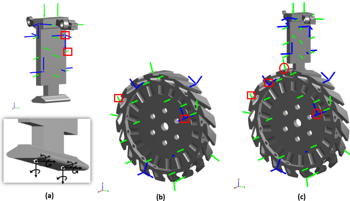
Fig. 7: The geometric models of the blade and disk showing the impacts' positions. The blue arrows denote the response channels (sensors) and the green arrows denote the impact points. The markers (squares and circles) indicate the DoF used to validate the SEMM method to be discussed in Section 4. The interface consisting of two virtual points is depicted on the blade geometry.
