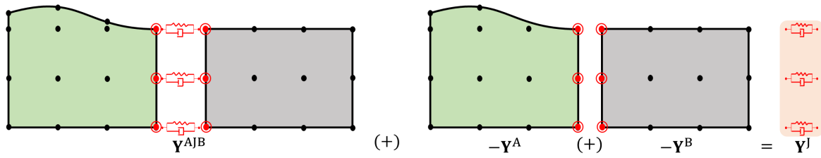
Fig. 3: Identification of the joint \mathbf{Y}^J is done by coupling the assembled structure's admittance \mathbf{Y}^{AJB} and fictitious admittances of the substructures \mathbf{Y}^A and \mathbf{Y}^B . The compatibility condition reads the same as in the case of coupling the joint in Fig. 2 (standard interface).
