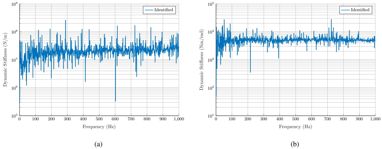
Fig. 12: The identified dynamic stiffness of the actual joint for: (a) translational DoF (b) rotational DoF
