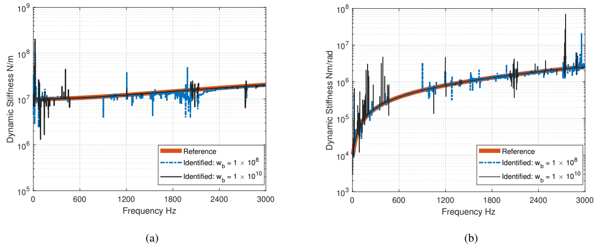
Fig. 9: The reference and identified dynamic stiffness of the dummy joint for: (a) Translational DoF (b) Rotational DoF on one of the two virtual points depicted on the blade in Fig. 6a. The identified stiffness plots are obtained after three iterations. In the first iteration, no initial guess was used i.e. the substructures were left uncoupled.
