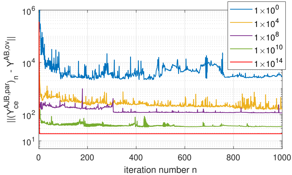
Fig. 13: Effect of weights on the convergence of Euclidean norm of the expansion error between the coupled parent model and the measured overlay model. The physical boundary DoF \mathbf{u}_b are weighted while computing the pseudo inverses, as per Eq. (21) and Eq. (22).
