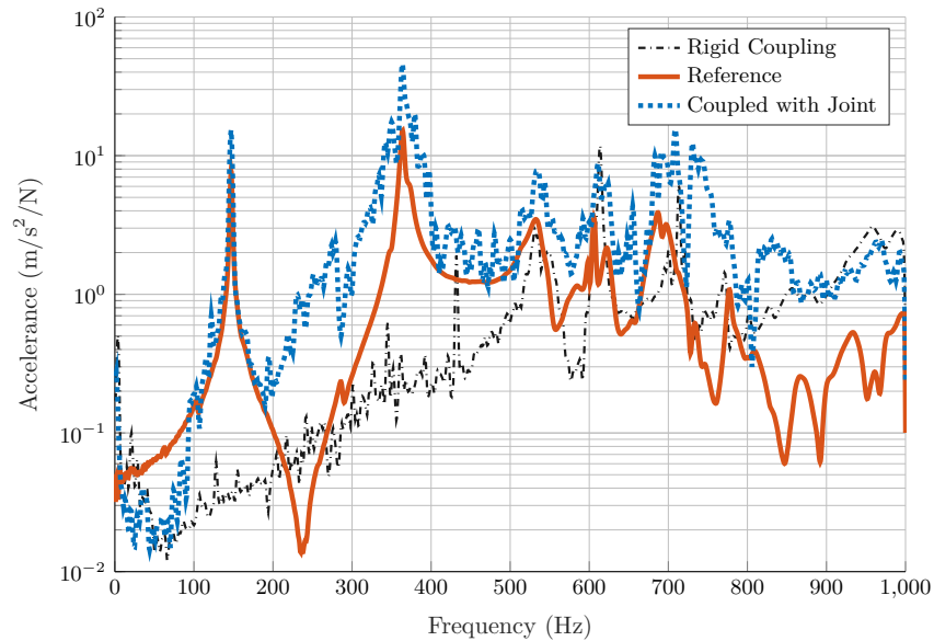
Fig. 11: The on-board validation of the joint. The solid validation line is a measured FRF of the full-system. This FRF (at the DoF marked with squares in Fig. 7c) has not been used to identify the joint. The blue dotted line indicates the coupled results (with the joint identified by the SEMM procedure). The dash-dotted black line is the would-be rigid coupling (without joint). The coupled results are not in good agreement with the full-system reference FRF but outperform the rigid coupling.
