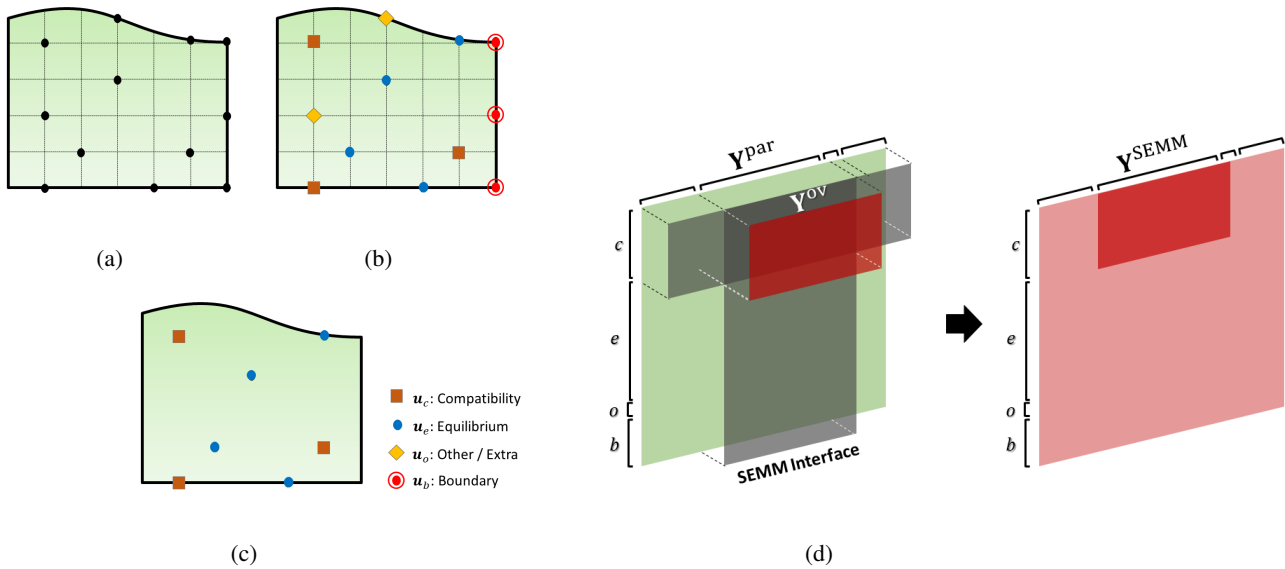
Fig. 4: (a) The reduced HCB model containing only master DoF set \mathbf{u}_m . This is used as a parent model of the substructure. (b) The master DoF set is labelled according to the classification defined. (c) The overlay model that provides dynamics to the parent model. (d) Block matrix illustration of SEMM. \mathbf{Y}^{\text{par}} is divided in four DoF sets vertically and horizontally.
