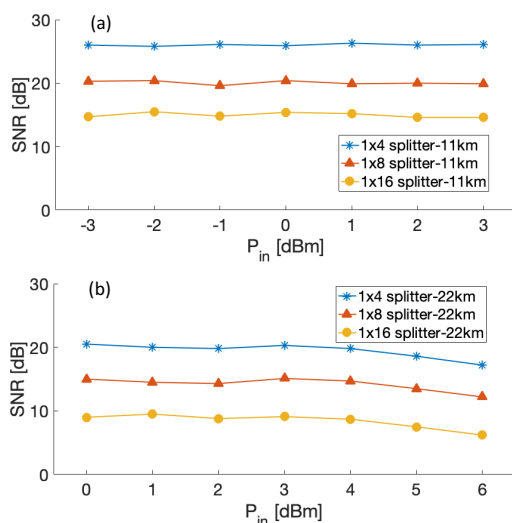
Fig. 4 SNR vs input sensing power P_I for 3 splitting ratios. a) 11 km and b) 22 km PON link.
