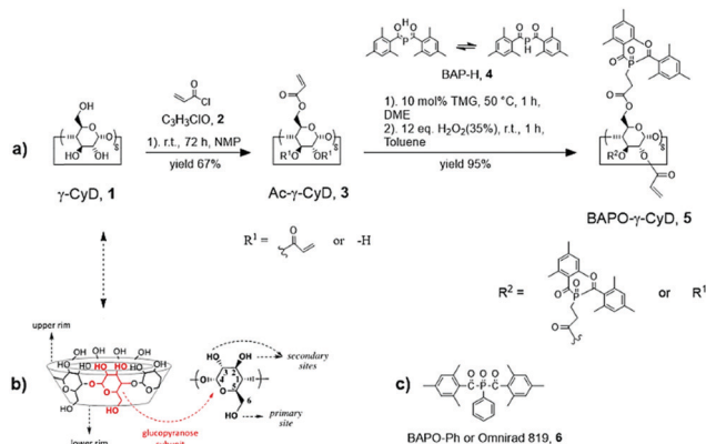
Fig. 1 (a) Synthetic route of multi-photoactive BAPO- \gamma -CyD 5 . (b) Chemical structure of \gamma -cyclodextrin ( 1 ) and commercial phenylbis(2,4,6-trimethylbenzoyl)phosphine oxide (BAPO-Ph or Omnirad 819, 6 ).
