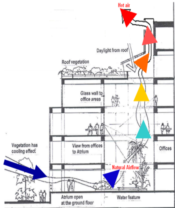
Fig. 34 Section shows passive and hybrid cooling strategies using water wall and roof chimney.
