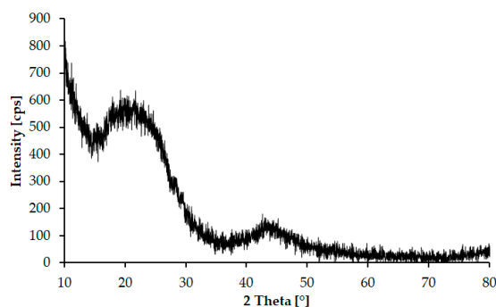
Figure 4. XRD pattern of Ultem 9085 solid residue obtained after thermal degradation.
