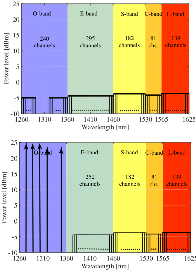
Fig. 5: Considered system configurations: a) Full MBT; b) O-band off, Raman in O-band, E → L-band.
