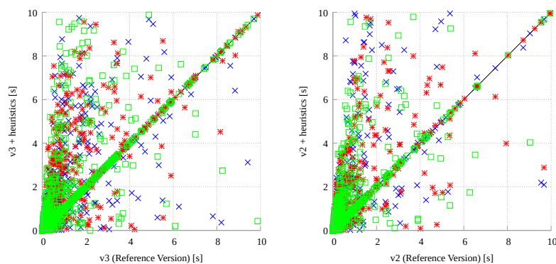
(a) Effect of the heuristics on the sequential version v3 . (b) Effect of the heuristics on the parallel version v2 .
