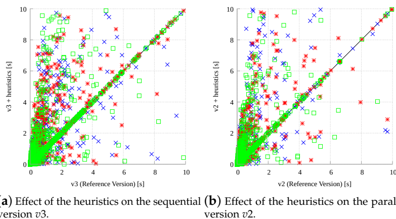
Figure 8. Running times for different heuristics (reported on the y-axis) implemented within the sequential (a) and parallel (b) version, and reported on the x-axis.
