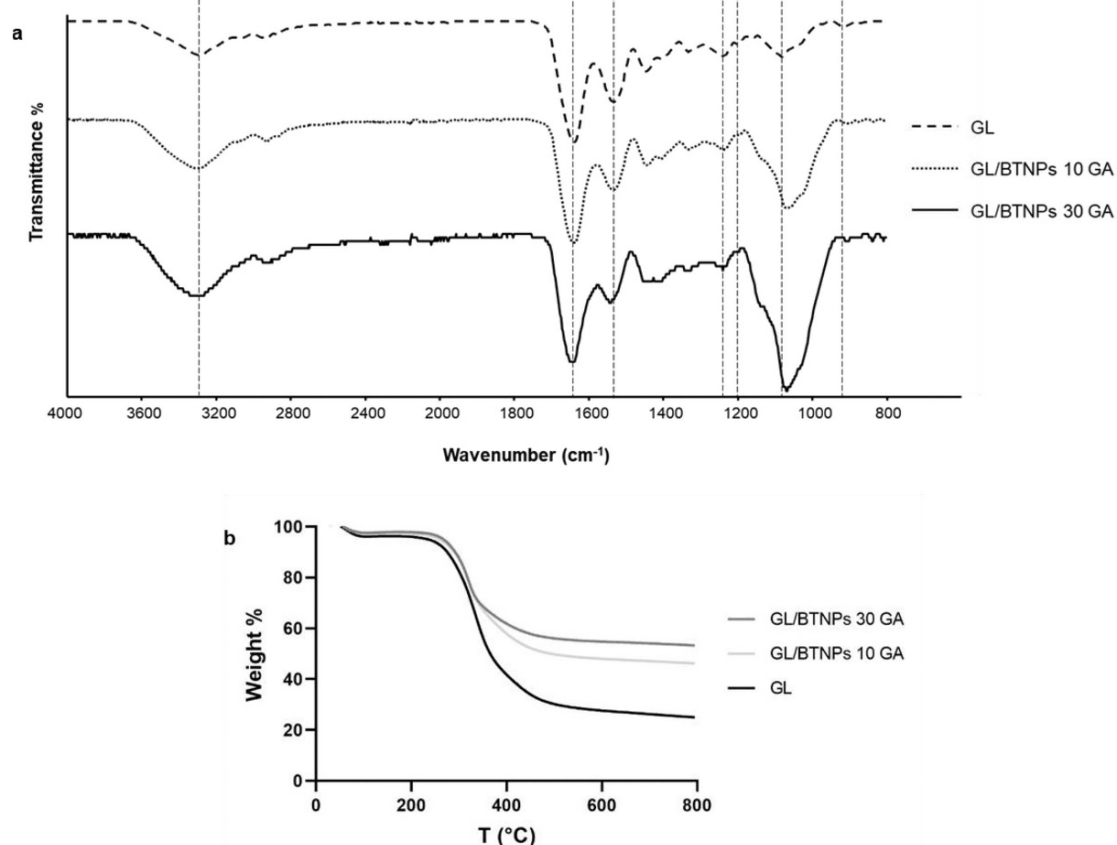
Figure 5. (a) FTIR-ATR spectra and (b) TGA of GL, GL/BTNPs 10 GA and GL/BTNPs 30 GA.
