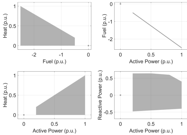
Fig. 3. Example of CHP capability/feasibility set for different bidimensional energy vector spaces.
