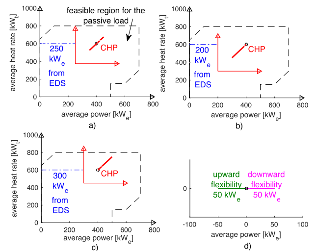
Fig. 20. Flexibility region starting from a given electricity and heat demand. (a) Reference case for the usage of the CHP. (b) Maximum reduction in the average power taken from the EDS. (c) Maximum increase of the average power taken from the EDS. (d) Upward and downward flexibility.
