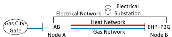
Fig. 10. Test system 2 to demonstrate multienergy network-related constraints and flexibility features.
