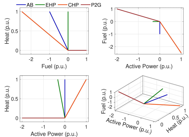
Fig. 5. Individual operational characteristics of AB, EHP, CHP, and P2G units in (top left) F-H, (top right) P-F, (bottom left) P-H 2-D planes, and (bottom right) P-F-H 3-D space.
