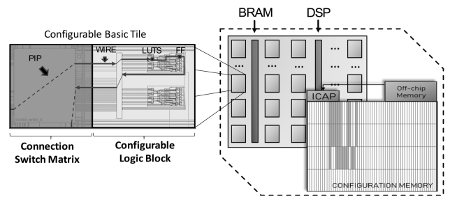
FIGURE 1. Overview of the current FPGA architecture: on the left the basic Tile unit is shown, with detail of the programmable resources and their functions; on the right the two layers fabric is schematized with the configuration memory layer and the programmable resource layer integrated with hardwired resources.
