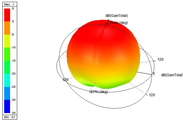
Fig. 9. Simulated gain of the antenna at the maximum graphene resistance of 3500 \Omega/\text{sq.}
