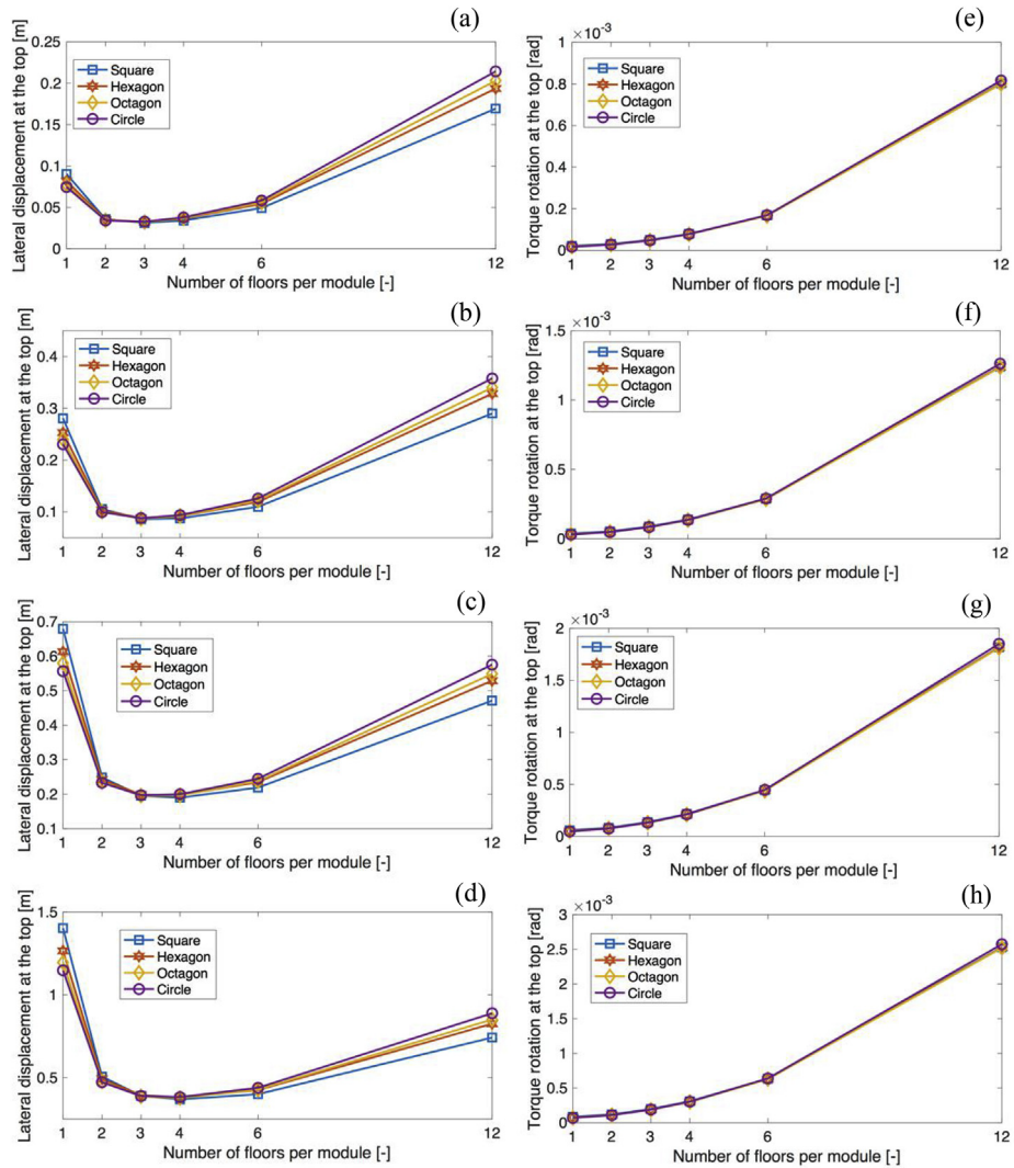
Fig. A1. Displacements (a-d) and torsional rotations (e-h) for the four buildings – Variable cross-sectional area.
