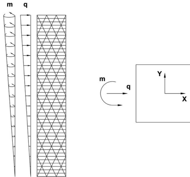
Fig. A2. Reverse triangle load pattern: q refers to the distributed horizontal load, m to the distributed torque moments.
