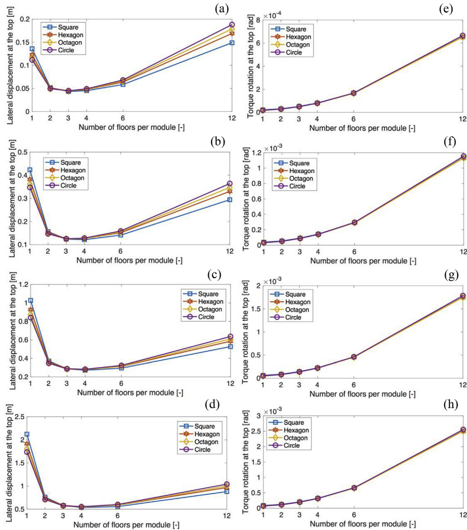
Fig. A3. Displacements (a-d) and torsional rotations (e-h) for the four buildings – Reverse triangle load.
