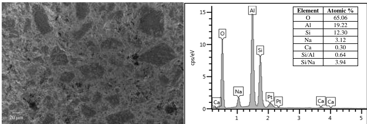
Figure 18: FE-SEM micrograph of as-prepared CH paste and EDS semiquantitative analysis (Pt was used for samples metallization)
