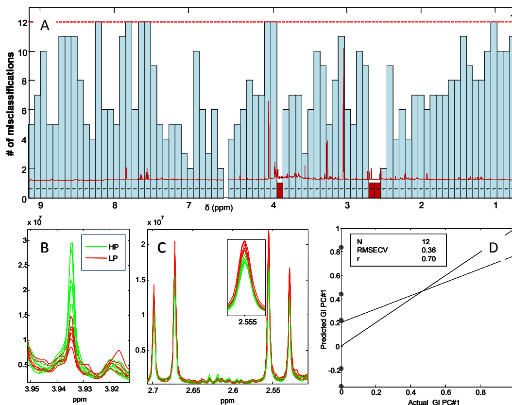
Figure 8. (A) iPLS-DA plot of classification of the high protein (HP) and low protein (LP) diet from 12 averaged ^1\text{H} NMR spectra of urine calculated on 80 intervals (full CV) showing the number of misclassification in absolute numbers. The 12 averaged spectra are divided into diet group (HP or LP) and gender at months 1, 3 and 6. The red dotted line indicates the number of misclassification for the full spectral model together with the number of PC. The RMSECV of the global model calculated with 1 LV's is markedly improved by the intervals colored red (3.86–3.94 + 2.45–2.72 ppm). These intervals include signals from creatine (3.93 ppm); (B) The RMSECV of the global model calculated with 1 LV's is markedly improved by the intervals colored red (3.86–3.94 + 2.45–2.72 ppm). These intervals include signals from creatine (3.93 ppm); (C) These intervals include doublets from citric acid (centered at 2.86 and 2.54 ppm); (D) The actual versus predicted plot shows almost perfect separation of the two diet groups using the selected intervals.
