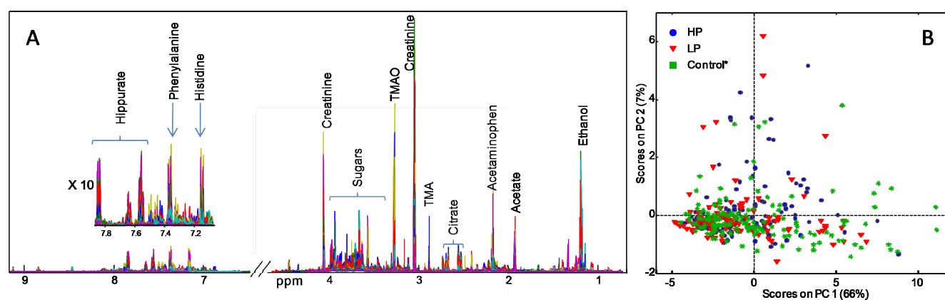
Figure 6. (A) ^1\text{H} NMR plot of the complete urine spectra ( n = 264 ) from 0.62–9.20 ppm including assignments of the most dominant signals; (B) PCA model of ^1\text{H} NMR spectra showing the overall variation between the samples. The PCA scores are colored according to diet group (high protein (HP), low protein (LP) and controls) showing no grouping at the individual level according to diet.
