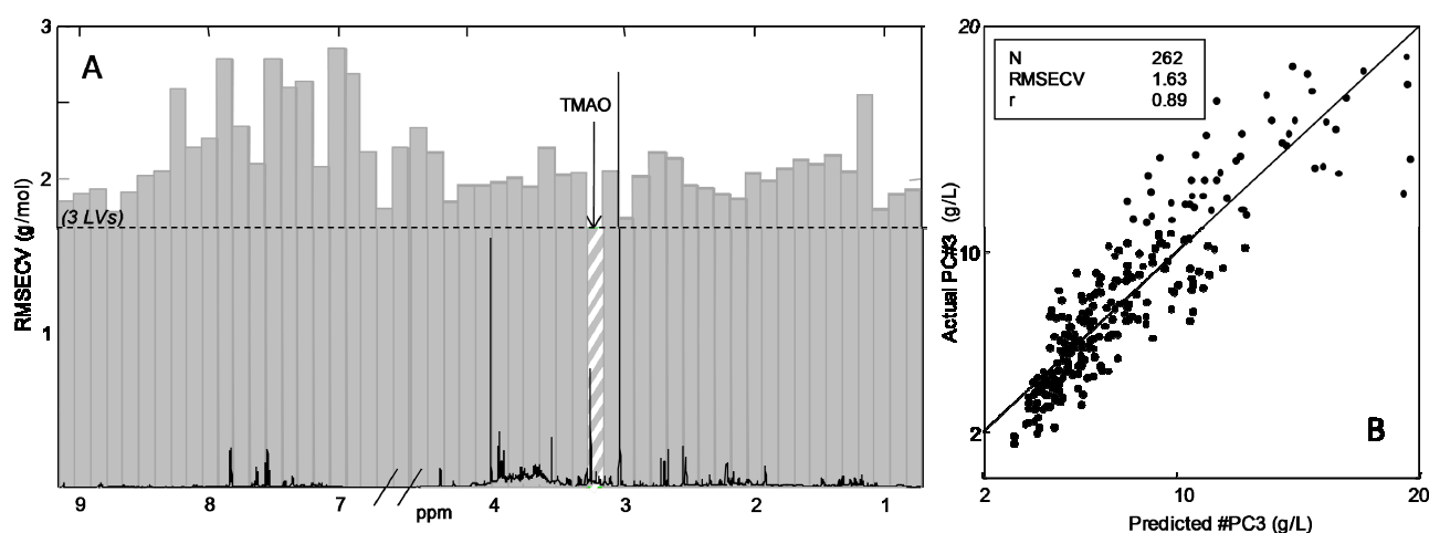
Figure 5. (A) iPLS plot of the prediction of nitrogen concentration (mmol/L) obtained on ^1\text{H} NMR spectra of urine using 54 intervals (200 variables). The dotted line shows RMSECV (3 latent variables (LV's)) for global model. The interval (3.17–3.29 ppm) containing signal from trimethylamine- N -oxide (TMAO) shows the lowest prediction error; (B) Predicted versus measured plot of PLS model calculated on the hatched intervals using 3 LV's.
