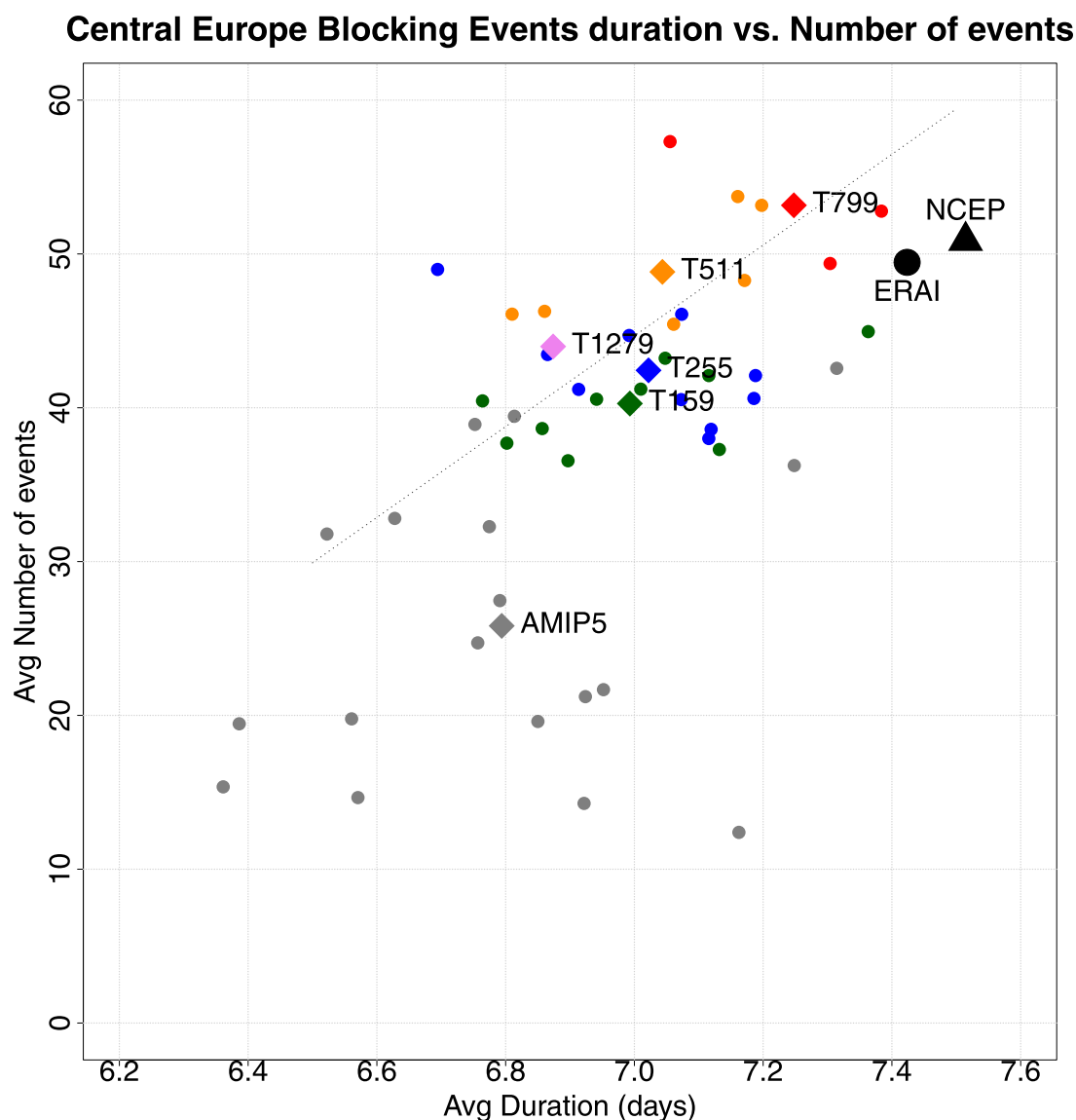
Figure 10. Blocking events duration versus number of blocking events averaged over the European sector as shown by Figure 1f. Each dot is an ensemble member, diamonds are the ensemble mean. The black dot is ERA-Interim, black triangle is NCEP/NCAR. The linear regression of the EC-Earth ensemble means is shown by the dashed line.
