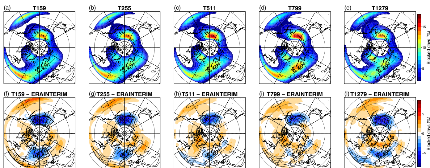
Figure 1. (a–e) DJFM 1979–2008 blocking events (blocked days) for the EC-Earth ensemble mean at five different resolution. (f–i) EC-Earth model biases (colors) against ERA Interim reanalysis (contours). Contours are drawn every 3%. Boxes identifying the different regions used in Figure 3 are shown in Figure 1f.
