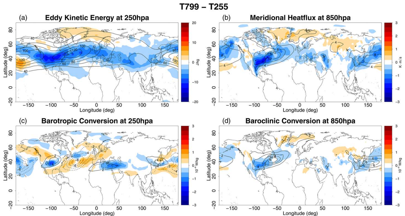
Figure 7. T799 ensemble mean minus T255 ensemble (colors) and T255 ensemble mean (contours) for (a) 250 hPa eddy kinetic energy; (b) 850 hPa transient heat flux ( \overline{v'T'} ); (c) 250 hPa barotropic conversion term ( \mathbf{E} \cdot \mathbf{D} ); and (d) 850 hPa baroclinic conversion term ( F ).
