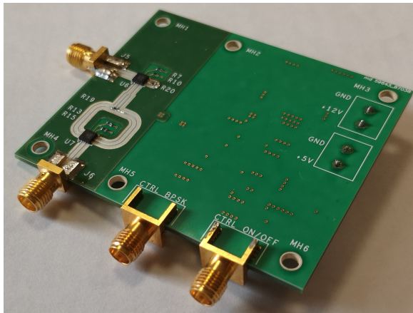
Fig. 3. Top view of the BPSK modulator board.
