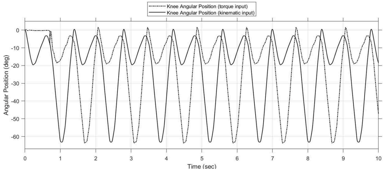
FIGURE 8 | Comparison between kinematic input of the Figure 3 and kinematic output giving torques as input.
