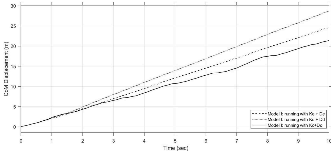
FIGURE 10 | Comparison of performances using Model I during running and using different stiffness and damping values for K_1 : K_c + D_c, K_d + D_d , and K_e + D_e .
