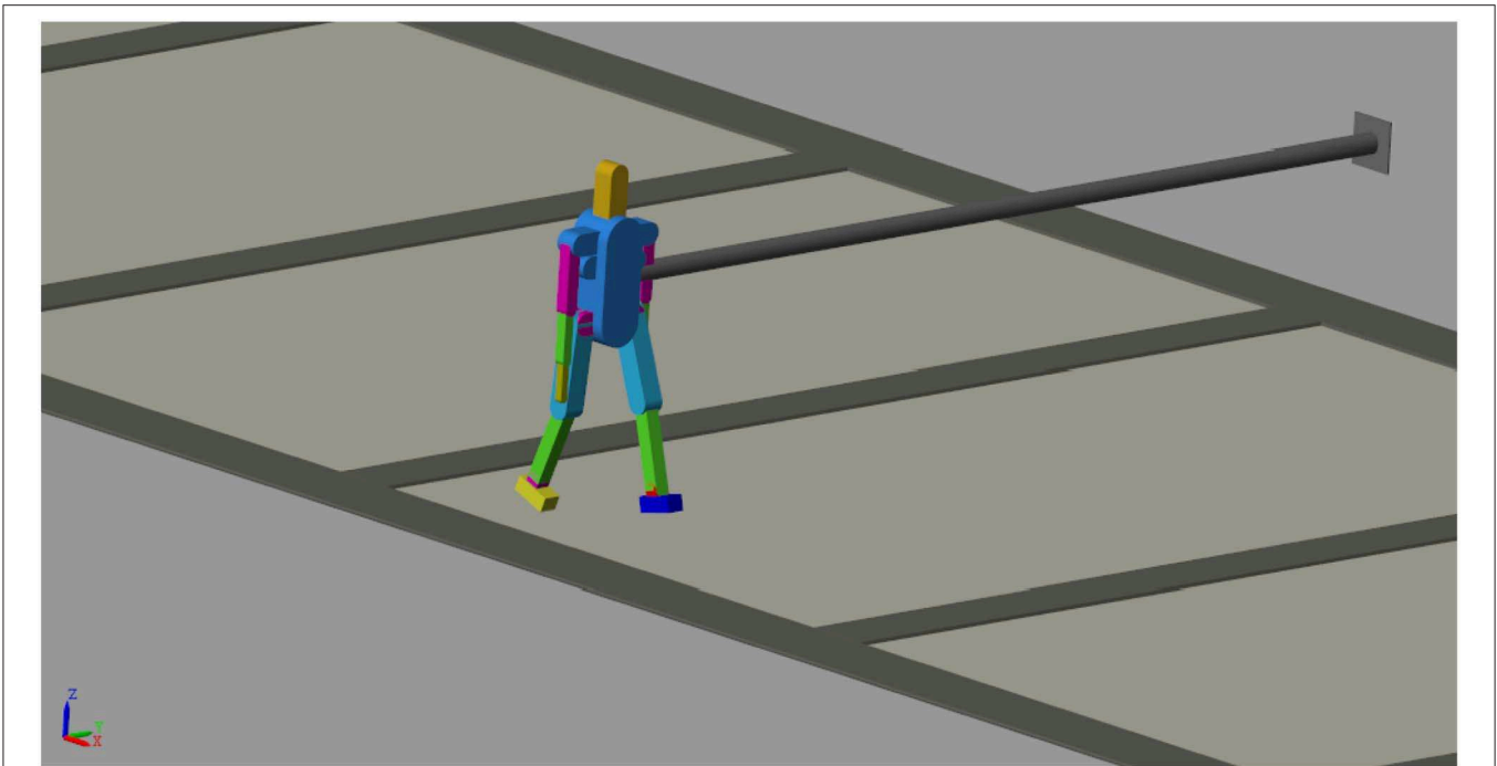
FIGURE 1 | Biped robot virtual model.
