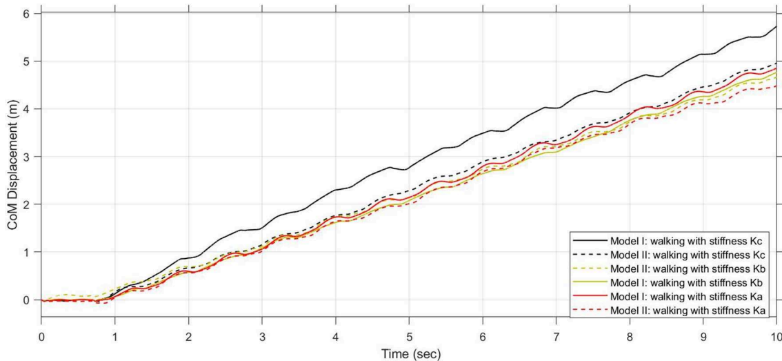
FIGURE 9 | Comparison of performances between Model I and Model II, during walking and using different stiffness value for K_1 : K_a, K_b , and K_c .
