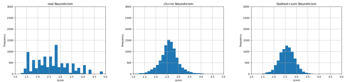
Figure 10. Neuroticism: Histograms representing data distribution of gold standard on the left, our model result in the middle, and previous state of the art by Carducci et al. [8] on the right.
