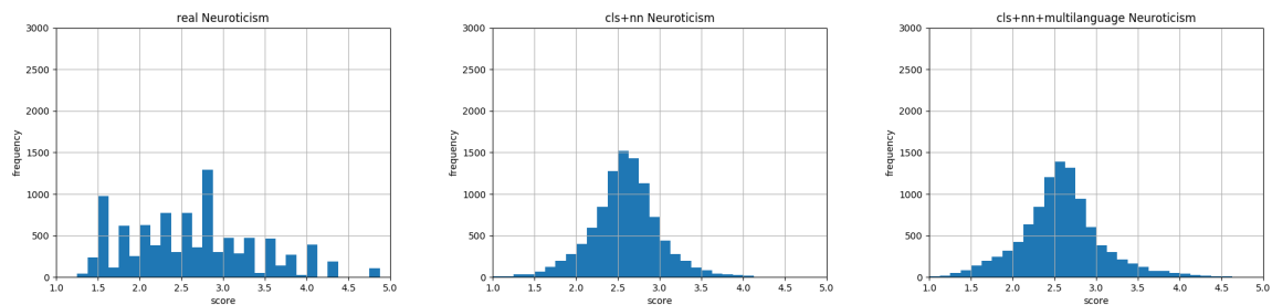
Figure 15. Neuroticism: Histograms representing data distribution of gold standard on the left, our English model result in the middle, and our multilingual model result on the right.
