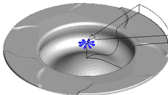
Figure 4. Selected cylinder sector from the entire combustion bowl geometry.
