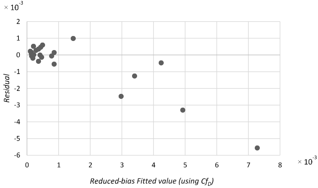
Figure 9 – DPU residuals versus reduced-bias fitted values considering Cf_D as the predictor (obtained from model (2) in Table 2) with copier assembly data (Su, Liu, and Whitney 2010).
