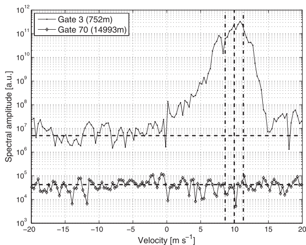
FIG. 4. Instantaneous rain and noise spectra measured during the convective cell at 1044:57 UTC at 0.75- and 15-km height, respectively. Horizontal dashed lines correspond to the noise level estimated using the routine processing, and vertical dashed and dotted–dashed lines show the mean Doppler velocity and the spectral width of the rain spectrum, respectively.
