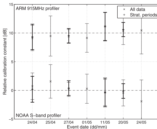
FIG. 11. Variability of event-based calibration constants of NOAA S-band profiler and wind profiler relative to the corresponding climatological ones.
