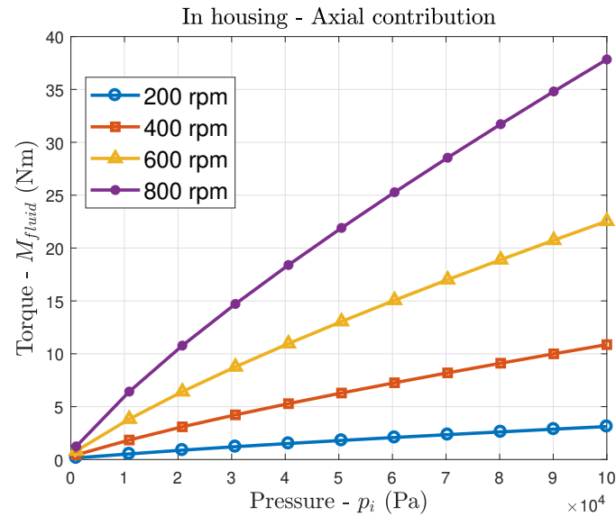
Figure 3. Axial component of the fluid friction torque as a function of the pressure at different rotational velocities.
