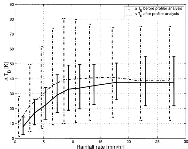
FIG. 7. Mean and std dev of the increase in T_{Bs} at 10.35 GHz for the cold front case at the CRM resolution as a function of the CRM rain rate at the ground. Note the reduction in the uncertainties in T_B after the profiler analysis.
