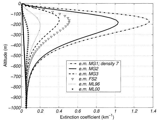
FIG. 4. Extinction profile at 10.35 GHz for a rainfall rate equal to 10 \text{ mm h}^{-1} .
