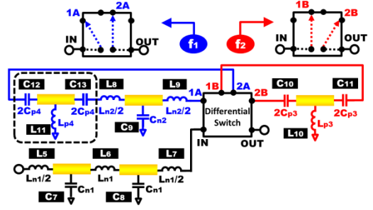
Fig. 3. Configurations of the -90° frequency agile branch at f_1 and f_2 .
