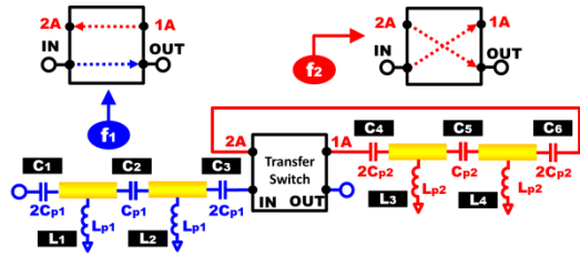
Fig. 2. Configurations of the +90° frequency agile branch at f_1 and f_2 .
