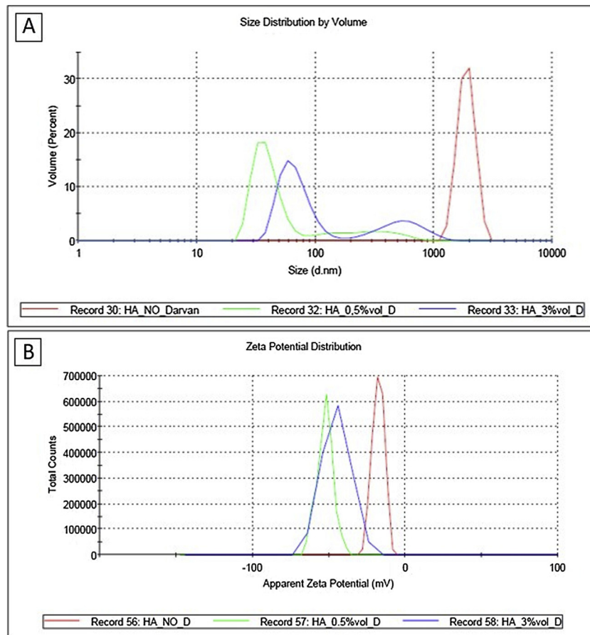
Fig. 4. DLS measurements of particle size (A) and Z-potential (B) of HA D suspensions containing 0 vol%, 0.5 vol% and 3 vol% of Darvan 821-A.
