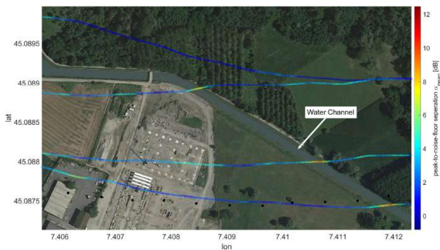
(b) Map display of the water channel, with the specular points superimposed on it. The colorgrade indicates the peak-to-noise-floor-separation \alpha_{mean} of the reflected signal.
