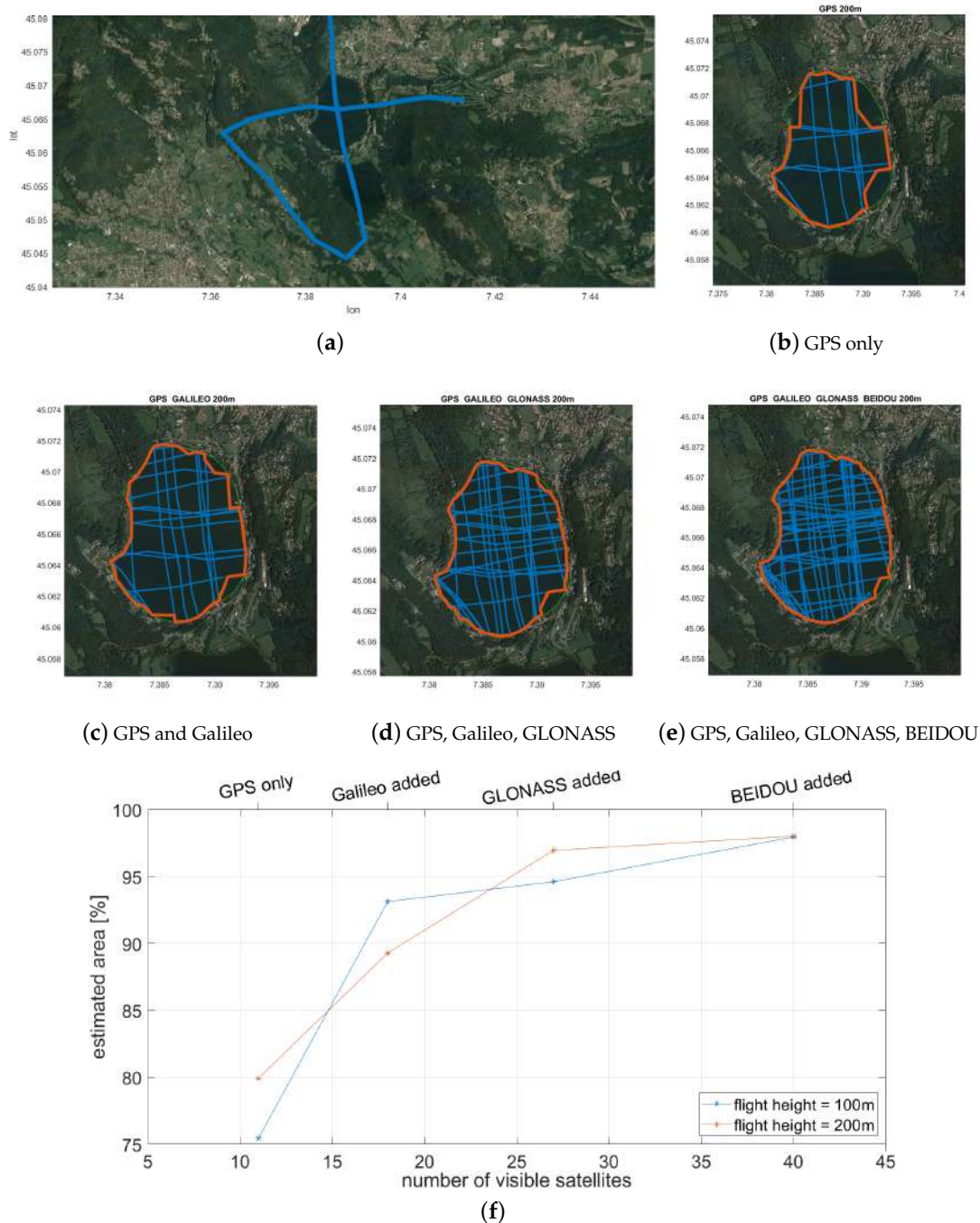
Figure 9. Simulation results of multi-GNSS reflections: (a) the sensor trajectory considered, (b–e) the specular points lines using the different GNSS constellations, (f) the ratio between the estimated and the real area of the Northern Avigliana lake versus the number of satellites in view, two different heights of the sensor are considered.
