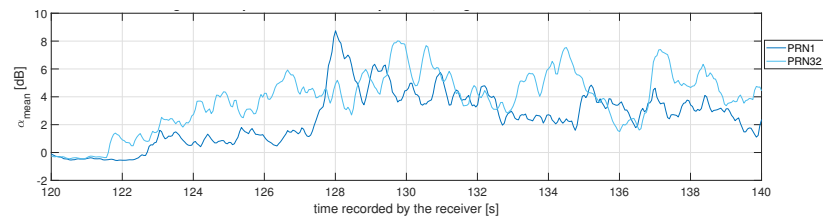
(a) Peak-to-noise-floor-separation \alpha_{mean} of the reflected signals when the specular points were over the river for PRN 1 and PRN 32.
