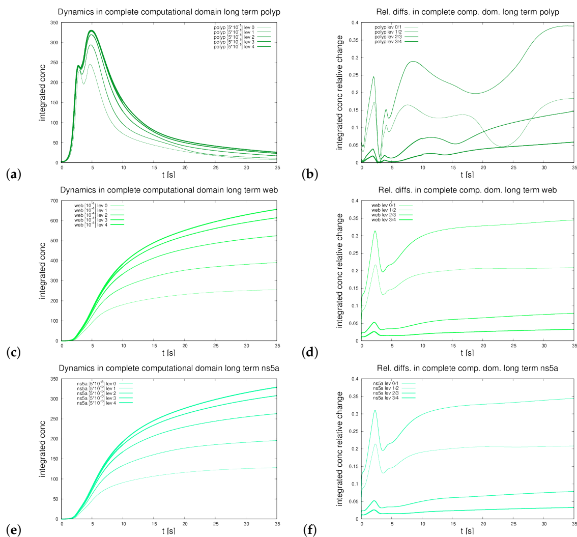
Figure A1. Development of integrated concentrations within complete computational domain under spatial refinement from level 0 (base level, direct reconstructed geometry) up to level 4 and relative differences respectively for concentrations of viral proteins. From top to down: Polypeptide, web protein, and NS5a. Left shows absolute values, while right shows relative differences. In detail: (a) Polypeptide absolute values for different grid refinement levels, (b) Polypeptide relative differences for different grid refinement levels, (c) web protein absolute values, (d) web protein relative differences, (e) NS5a absolute values, (f) NS5a relative differences.
