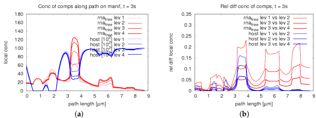
Figure A8. Grid convergency behavior of the concentrations of free HCV RNA and host factor along the long path around the ER and web surface at time t = 3 s: (a) concentrations at different levels; and (b) relative differences.
