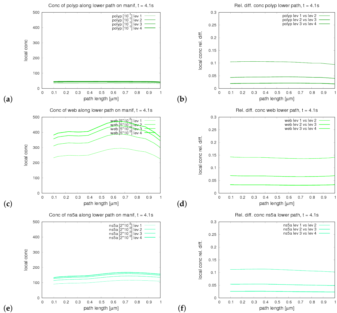
Figure A5. Variation of spatial refinement level for the 1D profiles of the concentrations around a web region. Lower sub path part two. Concentrations of viral protein components. (a) Polyprotein absolute values, (b) polyprotein relative differences, (c) web protein absolute values, (d) web protein relative differences, (e) NS5a absolute values, (f) NS5a relative differences.
