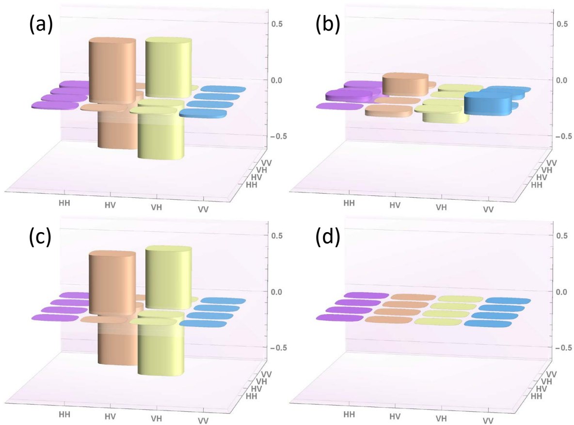
Figure 3. Tomographic reconstruction of the real (panel a) and imaginary (panel b) part of the reduced pseudo-density operator R_{13} = \frac{1}{4}(I - \Sigma_{13}) , related to the spatially maximally entangled state within the black hole, compared with the corresponding theoretically-expected counterparts (panels c and d, respectively).
