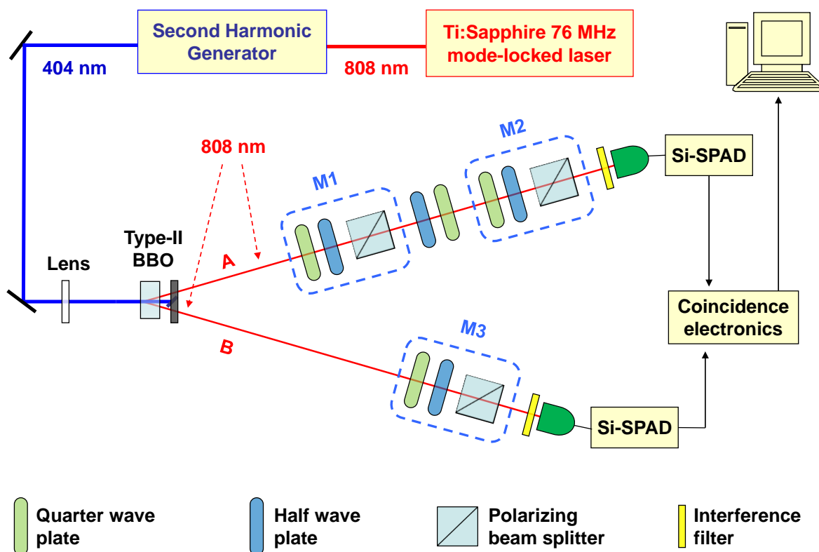
Figure 1. Experimental setup. A maximally entangled singlet state is generated by pumping a type-II Beta – BaB 2 O 4 (BBO) crystal. Two polarization measurements, M1 and M2 (at times t_1 and t_2 , respectively) are performed in sequence on photon A, while a single measurement (M3) is carried on photon B. Correlations among them certify entanglement monogamy violation for the whole pseudo-density operator (PDO) R_{123} in Eq. (2), describing the scenario of the spatio-temporal multi-partite entanglement (outside and inside the black hole) considered.
