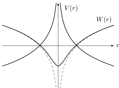
FIG. 1. Plots of V(r) = -\log |r| and a typical regularization W of -V .
