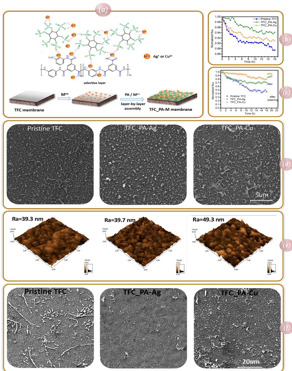
Figure 45. (a) Schematic diagram of TFC-PA-Ag and TFC-PA-Cu membranes fabrication procedure, water flux reduction during dynamic b) biofouling, (c) organic fouling tests with E. coli and sodium alginate as model foulants (d, e) SEM and AFM surface morphologies of pristine TFC and surface-modified membranes, and (f) SEM micrographs of the pristine TFC and surface-modified membranes (4 cycles of LBL assemblies) after incubation in E. coli suspension [289]. reproduced with permission from ACS Publications.
