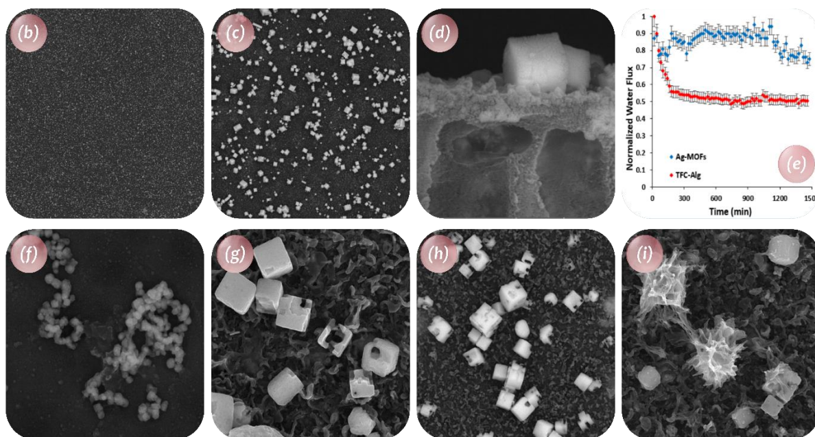
Figure 8. a) Schematic illustration of Ag-MOFs functionalized TFC membrane, b, c, d) surface and cross sectional FE-SEM images of in-situ functionalized Ag-MOFs TFC membrane, e) flux decline during dynamic biofouling test by E. coli of the nascent TFC and Ag-MOFs functionalized membranes, f) FE-SEM images after 6 h FO test, g) after 7 months soaking in water, g) after harsh sonication and after regeneration via the same procedure applied for initial in-situ surface functionalization [241]. reproduced with permission from Elsevier.
