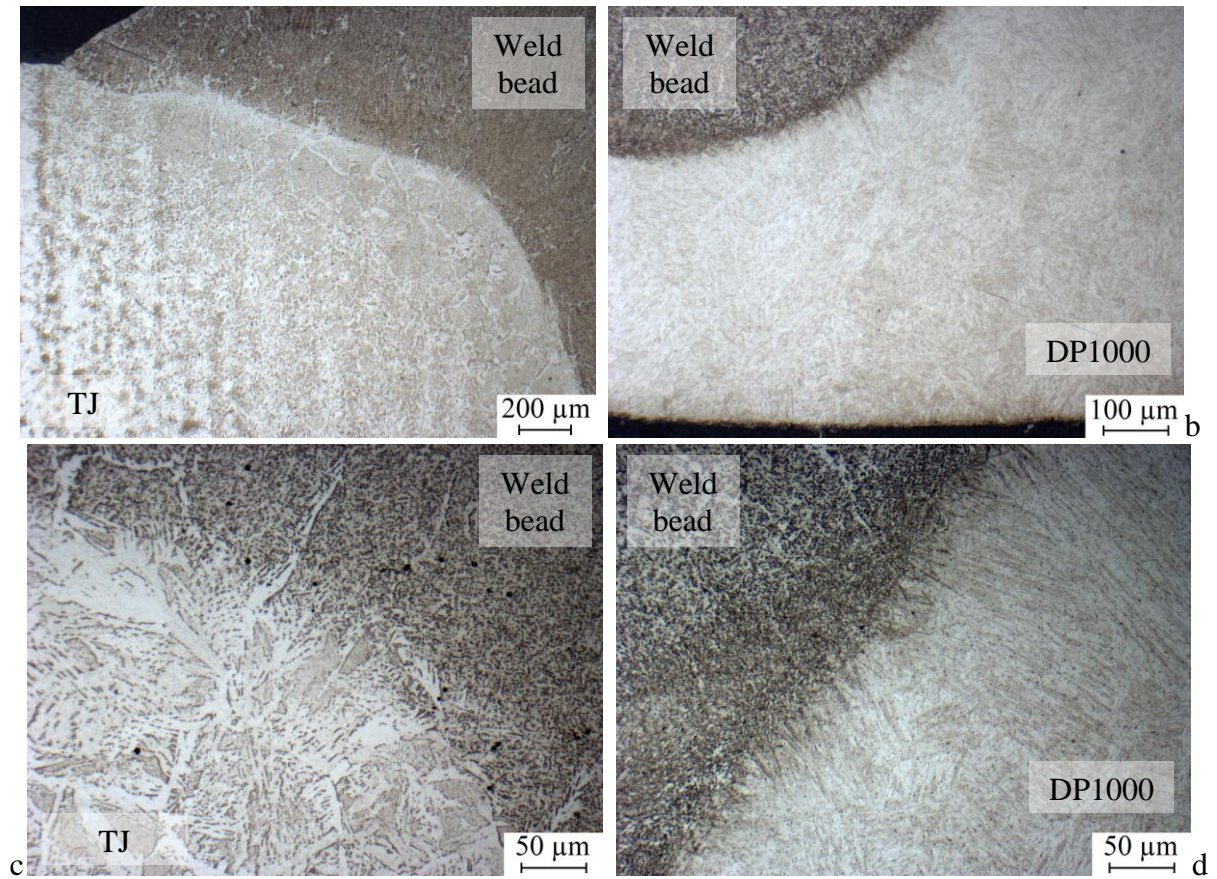
Fig. 8: Cross section of the weld between the DP1000 steel sheet and the steel side of the transition joint. Weld bead (dark) and HAZ on the transition joint side (a,c) and on the sheet side (b,d); increasing magnifications. Type C partial hybrid joint (the Al alloy side was not welded).
