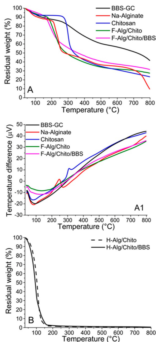
Figure 3. (A) Thermal gravimetrical analysis (TGA) and (A1) Differential thermal analysis (DTA) profiles of BBS-GC (black curve), sodium alginate (red curve), chitosan (blue curve), F-Alg/Chito (green curve) and F-Alg/Chito/BBS (magenta curve); (B) TGA profiles for hydrogels: H-Alg/Chito/BBS (solid curve) and H-Alg/Chito (dashed curve).
