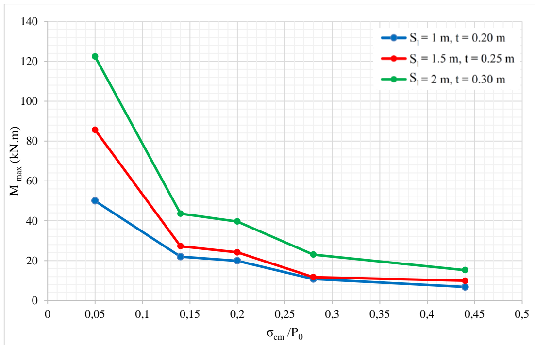
Figure 11. The average maximum bending moment for different rock masses. Key: S_l , longitudinal spacing between bolts; t , shotcrete layer thickness
