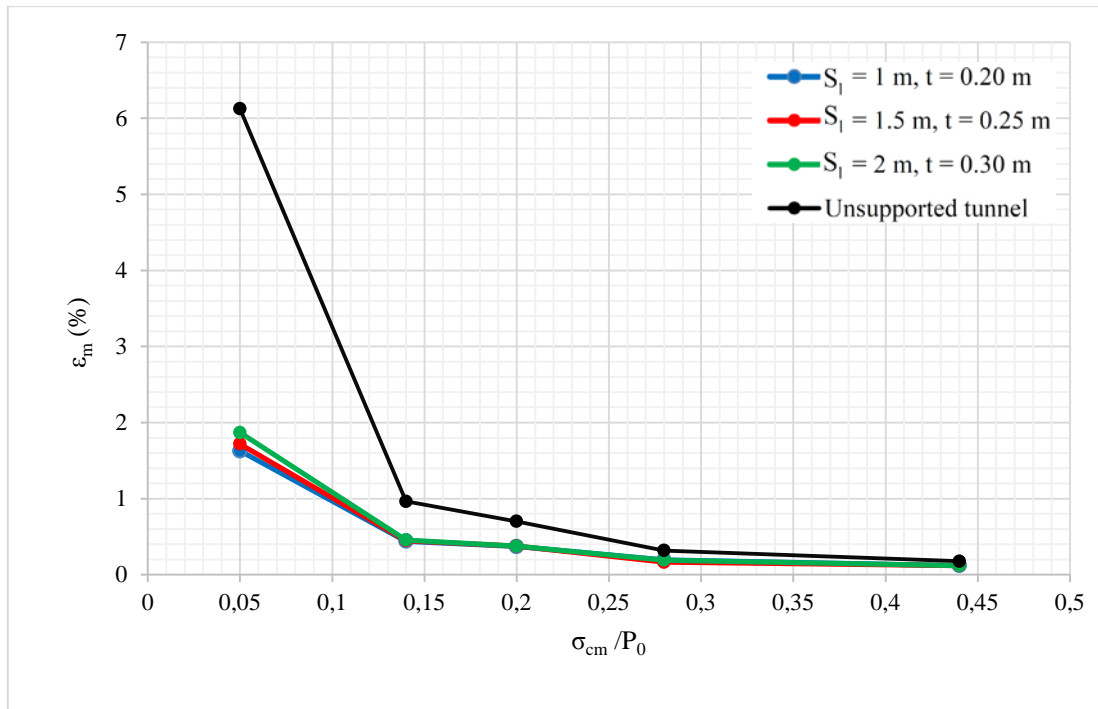
Figure 10. \frac{\sigma_{cm}}{P_0} vs \varepsilon_m (%) for unsupported and supported tunnels with fully grouted rockbolts and the shotcrete layer. Key: S_l , longitudinal spacing between bolts; t , shotcrete layer thickness
