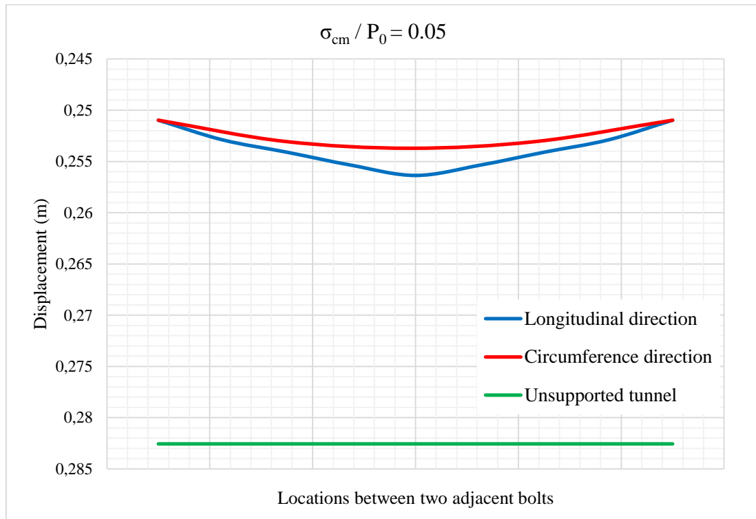
Figure 7. Tunnel surface displacements between two adjacent bolts ( S_l = S_c = 1 m, GSI = 25, P_0 = 13 MPa, \sigma_{ci} = 45.96 MPa)
