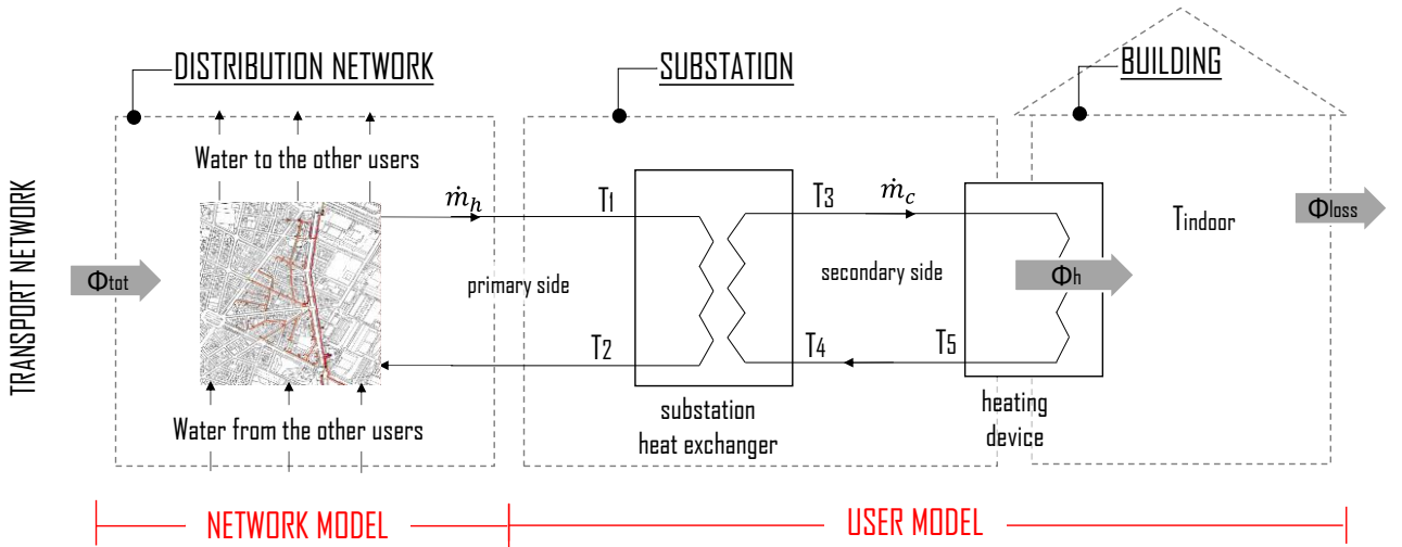
Fig. 3 Simplified scheme of the considered system.
