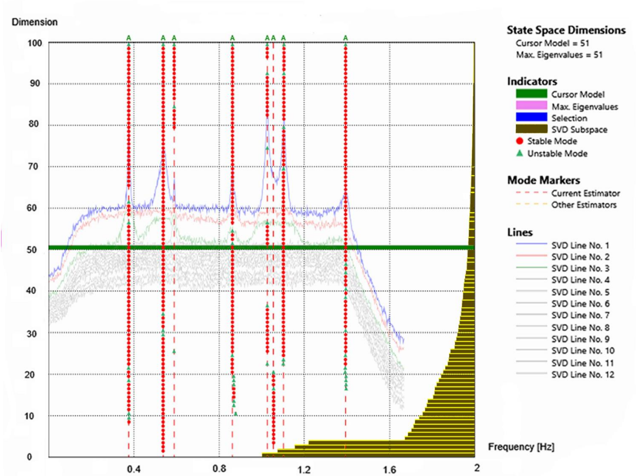
Fig.7 Stabilisation diagram
